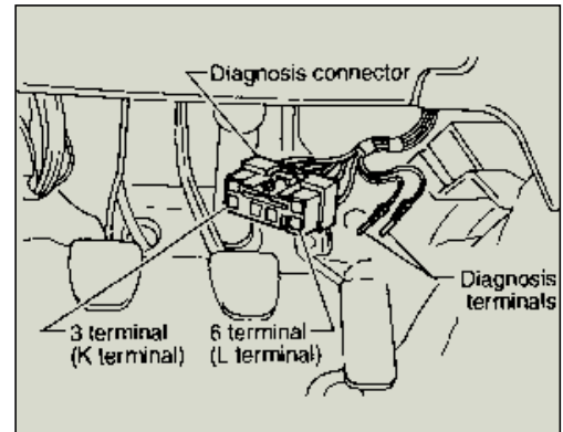
Diagnostic Connector
