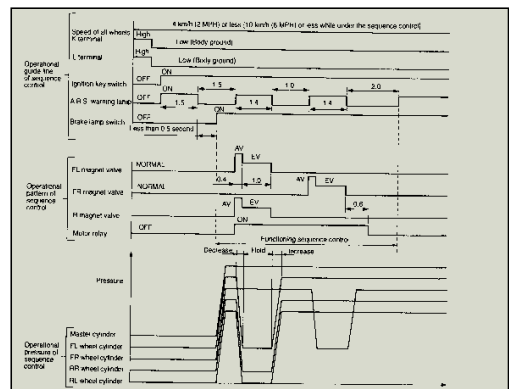
Sequence Control
