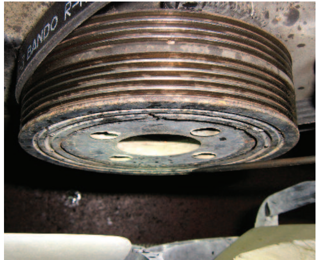
Perfectly normal harmonic balancer/crank pulley assembly, right?
