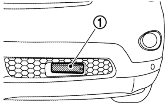
The main ICC sensor (1) also houses the computer used in determining how to control the rest of the vehicle based on sensor input.
