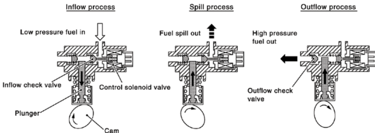
The ECM manages high fuel pressures by actuating the control valve solenoid and its one-way valve.
