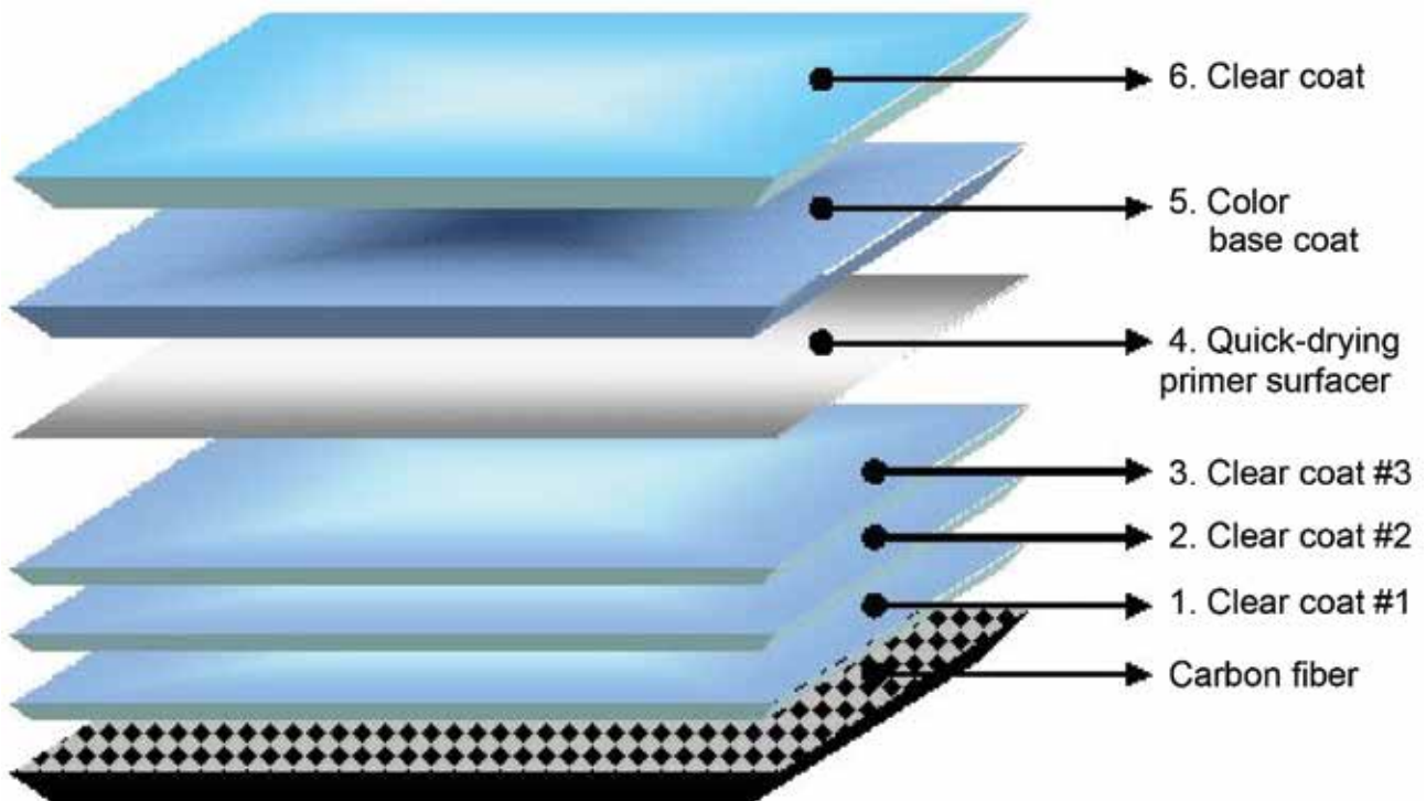
The light-colored body panels (trunk lid and front and rear bumper fascia) receive layers 4, 5 and 6 in the coating steps diagram, while the darker components receive only the clear (steps 1, 2 and 3).
