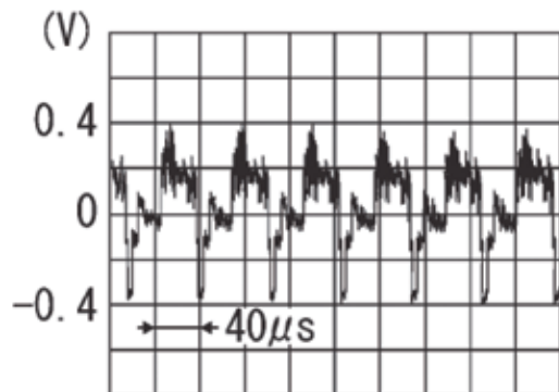
Reference values measured between the AV Control Unit terminal 62 (red wire) and ground, with the ignition on, in a 2011 Murano Z51 with base audio and color display installed should range between 0.4 and -0.4 V.
